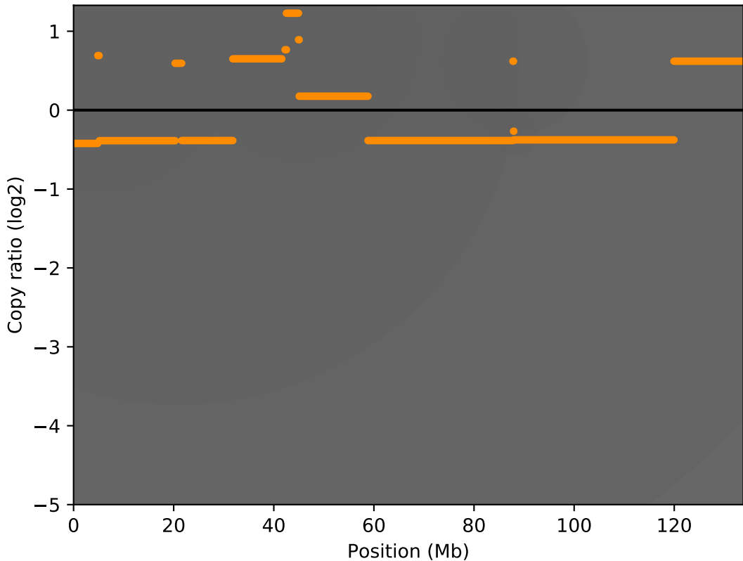
Exome_Tumor_sorted_mrkdup chr10
