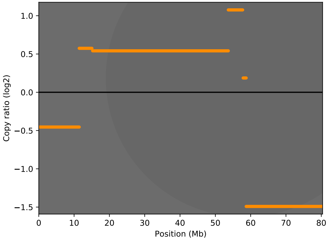
Exome_Tumor_sorted_mrkdup chr18
