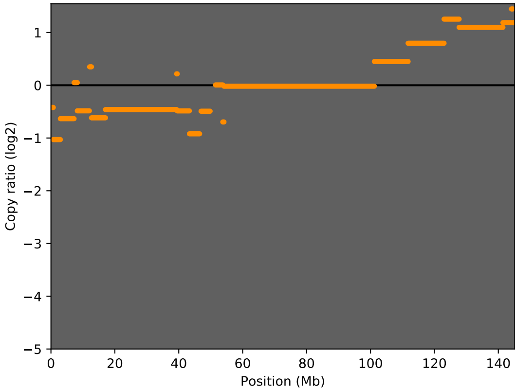
Exome_Tumor_sorted_mrkdup chr8
